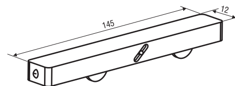
Tándem Regulable C-90106-03-0-1
